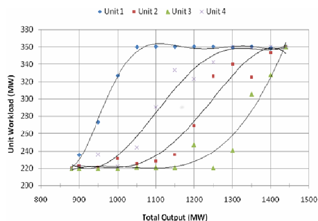
Fig. 2. Optimal unit loading distribution for the whole range of the generation capacity
