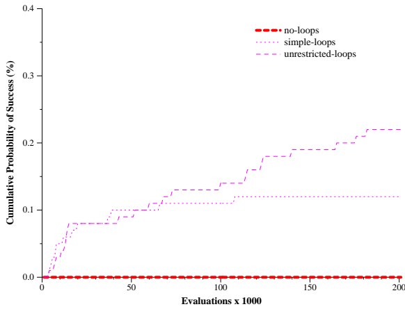
Fig. 3. Cumulative probability of success, modified ant problem, max-iterations=6, average of 100 runs, (the no-loops line is on the x axis)
