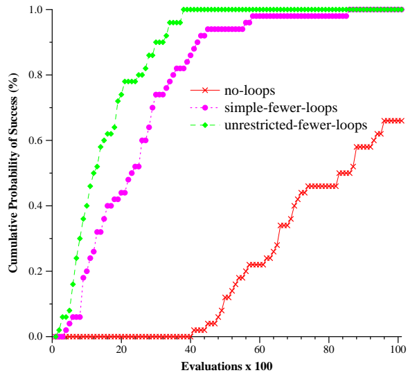
Fig. 12. Cumulative probability of success, sorting problem
