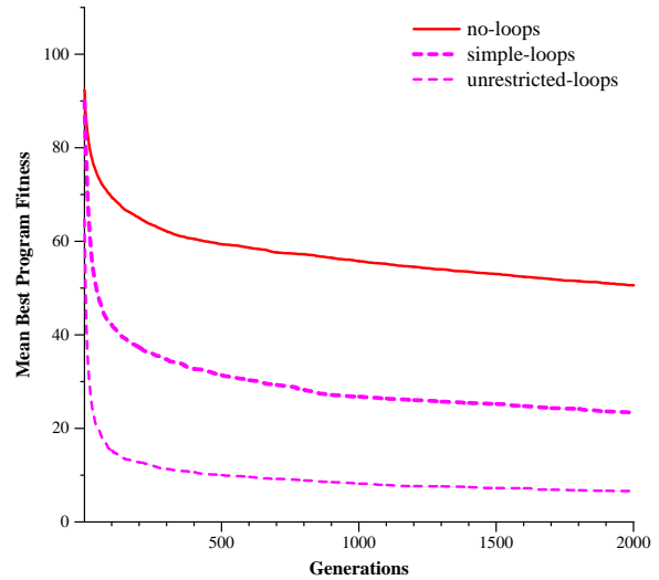
Fig. 2. Mean best program fitness, modified ant problem, max-iterations=6, average of 100 runs
