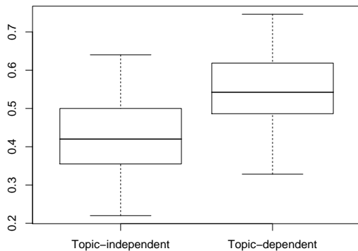
Figure 1: Classification accuracy: Topic-independent vs. topic-dependent
