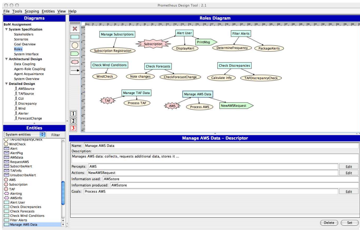
Figure 1. Screen-shot of PDT.
