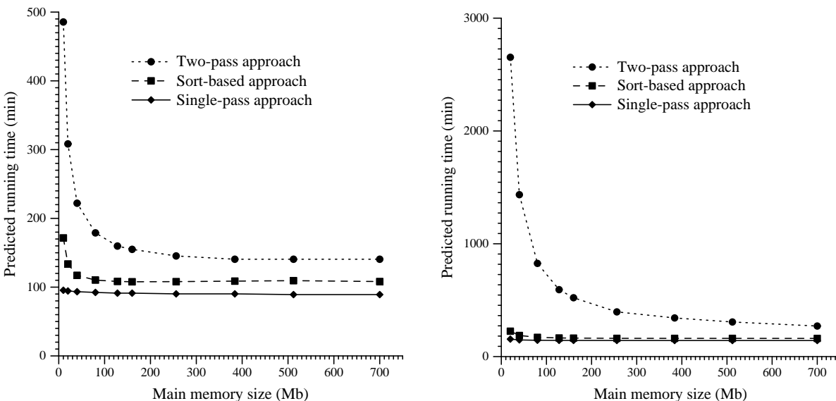
Figure 3: Predicted running times in minutes to construct a document-level inverted file on the left and a word-level inverted file on the right hand side for collection Web XX with varying main memory sizes, for the inversion approaches.
