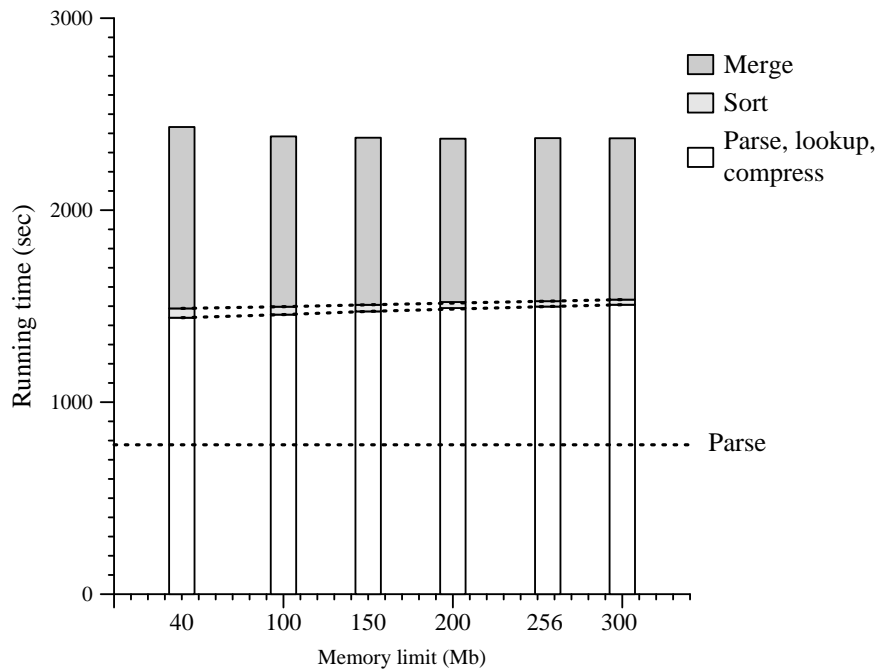
Figure 4: Break-up of the total elapsed time in seconds for constructing a word-level inverted file for Web V, with the single-pass inversion approach and a hash table lexicon, for different main memory limits. The total elapsed time consists of the time to parse, lookup, and compress postings, the time spent sorting the hash tables to create a sorted run, and the time to merge the runs. The total elapsed time for the parsing process is approximately 778 seconds.
