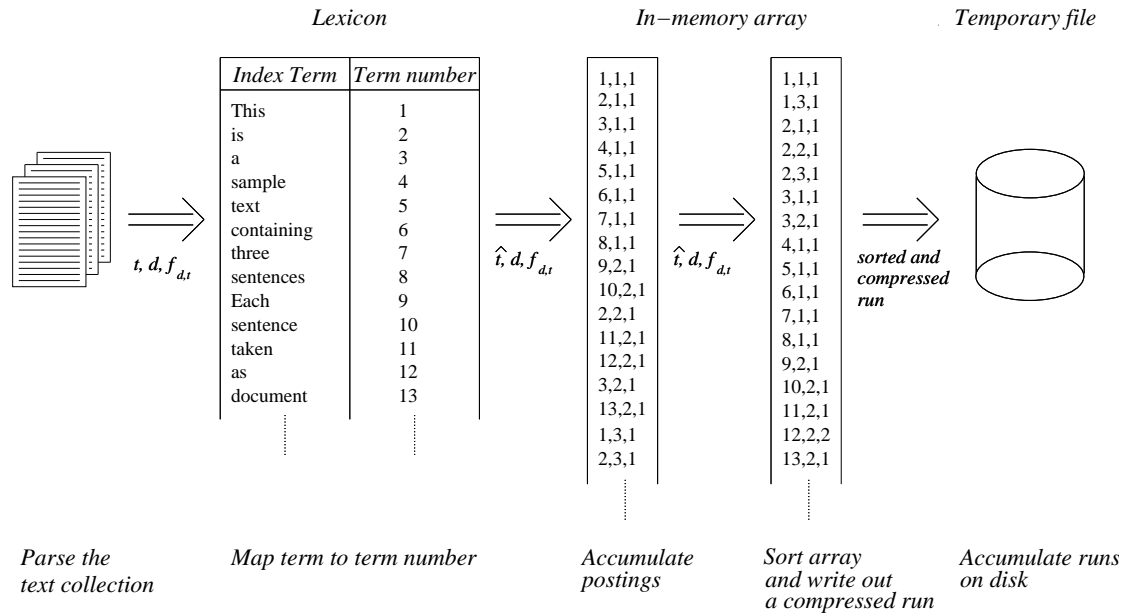
Figure 2: Constructing sorted and compressed runs during the sort-based approach.
