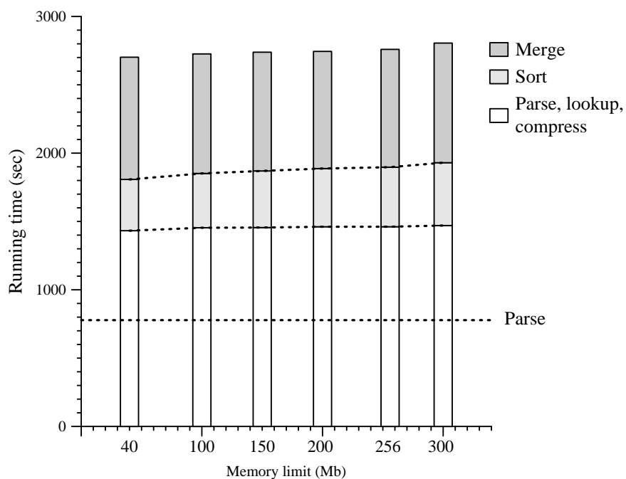
Figure 5: Break-up of the total elapsed time in seconds for constructing a word-level inverted file for Web V, with the sort-based inversion approach, for different main memory limits. The total elapsed time consists of the time to parse, lookup, and compress postings, the time spent sorting the accumulated postings, and the time to merge the runs. The total elapsed time for the parsing process is approximately 778 seconds.
