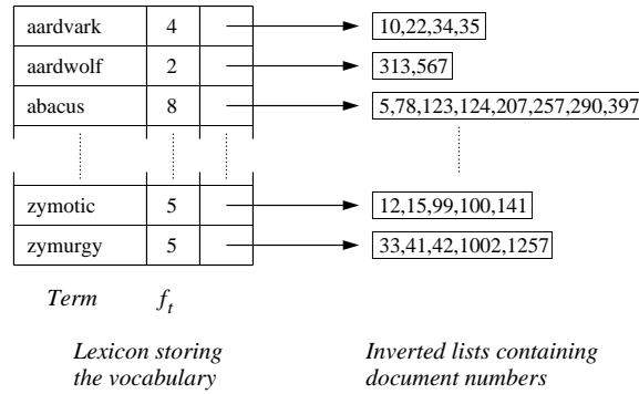
Figure 1: Structure of a simple inverted file. The lexicon maintains for each index term a reference to an inverted list on disk. An inverted list contains document numbers in ascending order.
