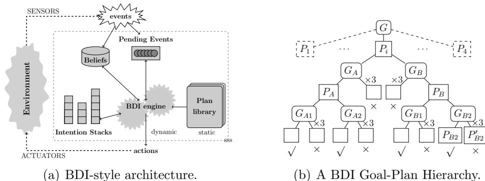
Figure 1: BDI Architecture and Goal-Plan Hierarchy.
